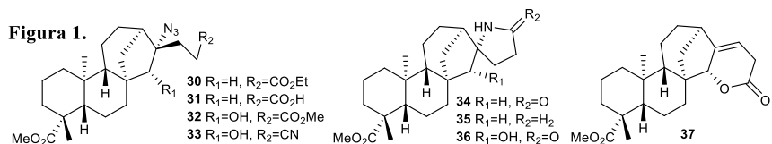
Schema 6. a) R-I, iPr 2 NH, 27 (cat.), hv; b) R 1 -I, RN 3 , iPr 2 NH, 27 (cat.), hv.
