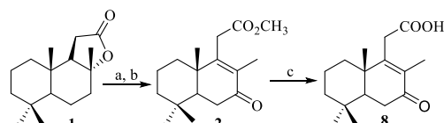
Schema 2. a. MeOH, H 2 SO 4 conc., Δ, 96 ore; b. LiClO 4 , MeOH, t.c., 7 ore, 63%; c. EtOH, KOH, 50°C, 3 ore, 79%.
