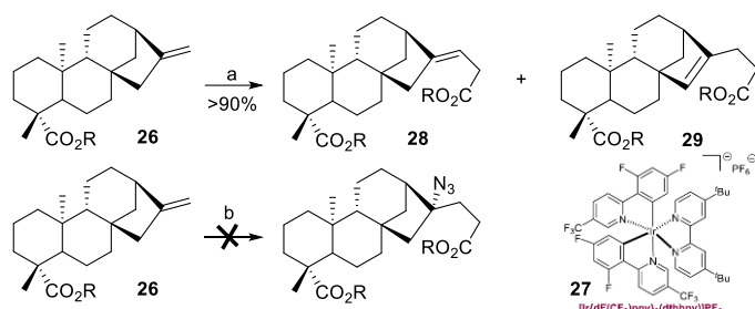
Schema 6. a) R-I, iPr 2 NH, 27 (cat.), hv; b) R 1 -I, RN 3 , iPr 2 NH, 27 (cat.), hv.
